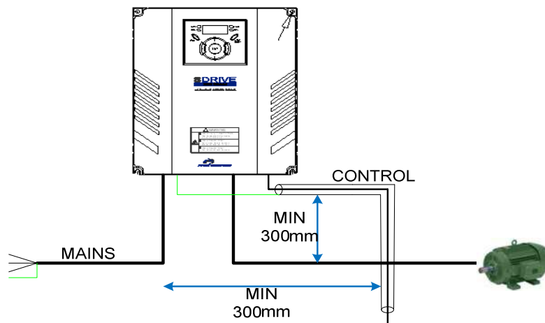
Figure 6 – Control Wiring
