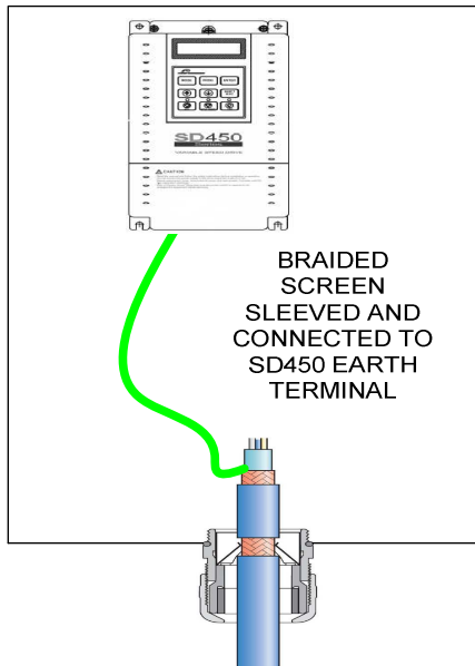
Figure 8 - Showing typical arrangement when SD450 is within MCC or Enclosure.
