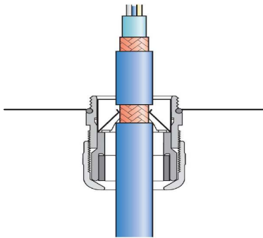
Figure 2 - Typical Gland Arrangement at Motor
