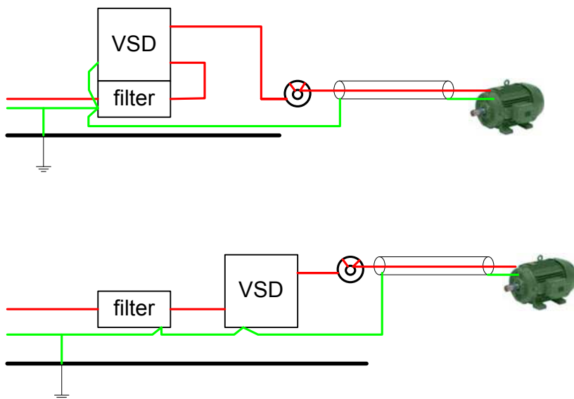
Figure 10– SD450 with First Environment RFI Filter (Footprint or External)
